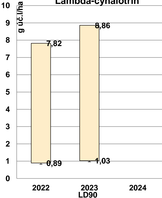
Lambda-cyhalotrin
